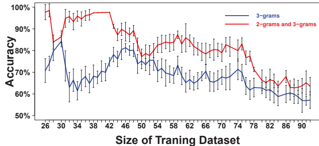
Figure 3: Average accuracy of decision trees applied to 3-grams, and combination of 2-grams and 3 grams for different size of training dataset using ten runs of 10-fold cross validation.
